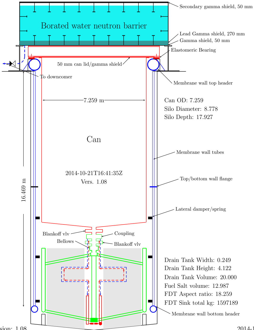
Figure 9: Cross-section of silo looking north
