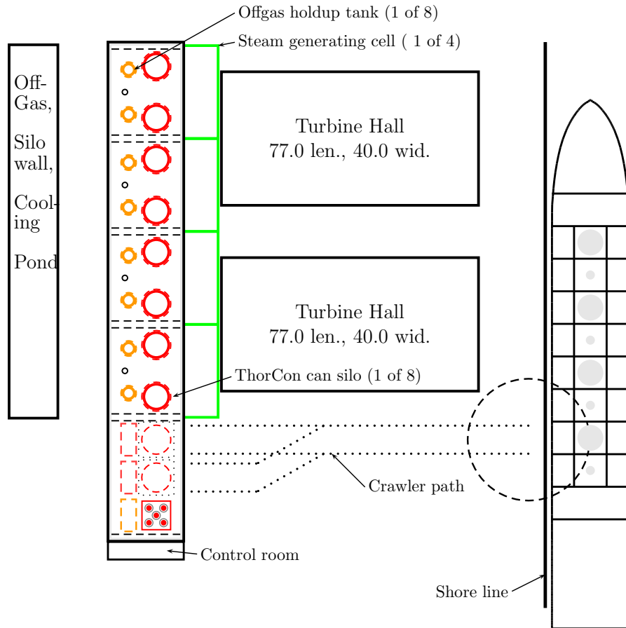
Figure 7: Site plan
